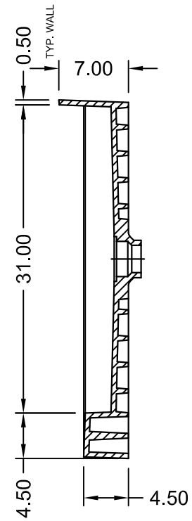
SECTION B-B
